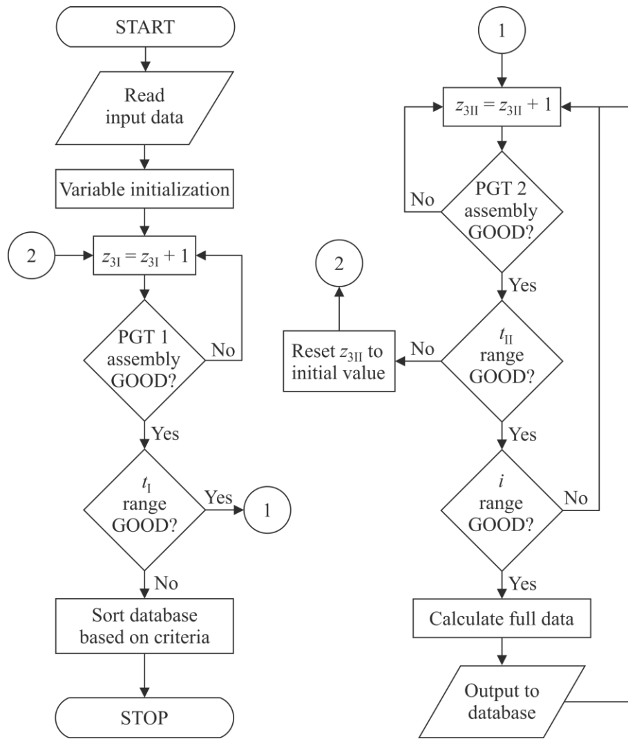
Figure 4. Flow chart of the DVOBRZ software.
