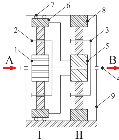
Figure 6. Kinematic scheme of S13WN planetary gear train.
