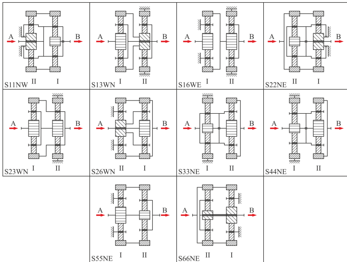
Figure 5. Applicable variants of single speed transmissions.
