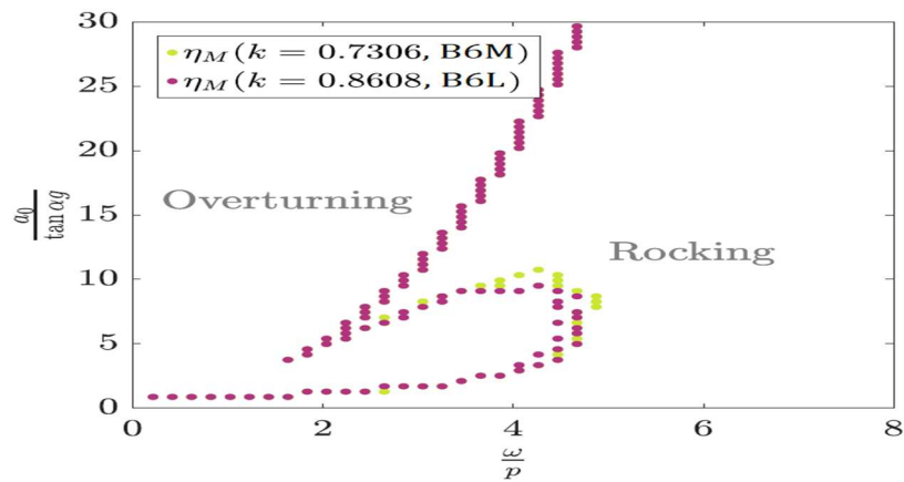
Figure 9. Stability graph for a single cosine wave acceleration excitation for blocks with \frac{h}{b} = 4.5 : B6M and B6L.
