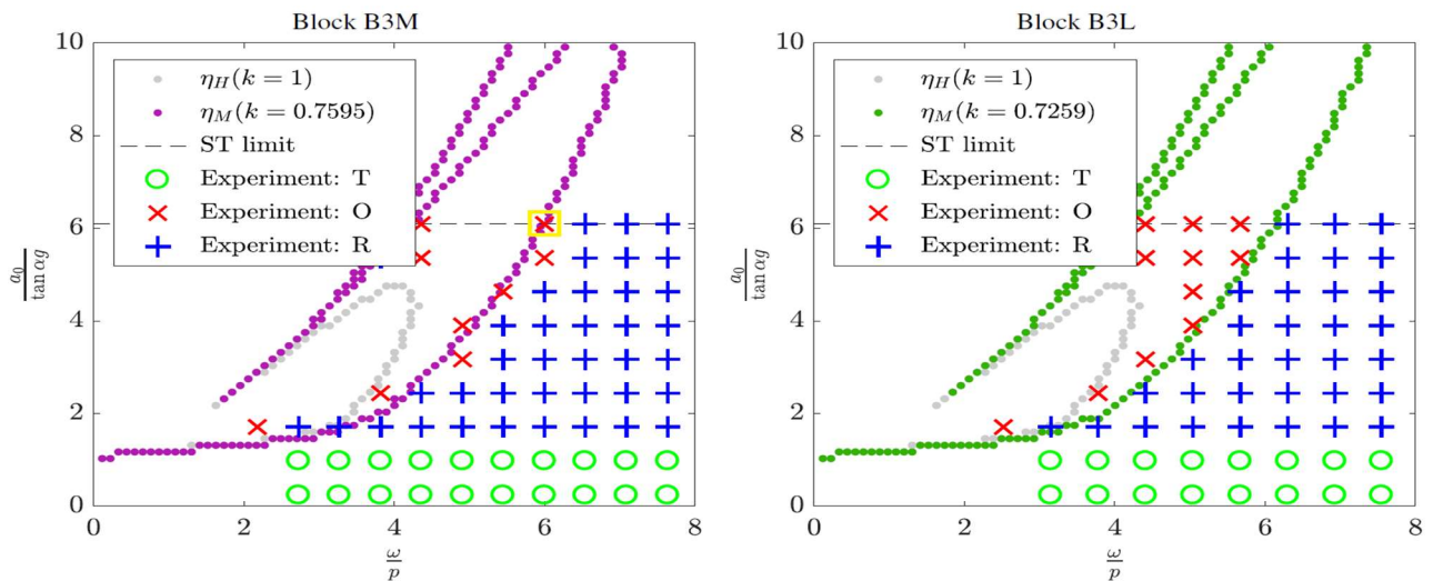
Figure 16. Stability graph due to a single sine wave for blocks B3M and B3L with \frac{h}{b} = 2.25 and exact parameter k for each block (T - translation, O - overturning, R - rocking).
