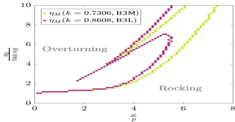
Figure 6. Stability graph for a single sine wave acceleration excitation for blocks with \frac{h}{b} = 2.25 : B3M and B3L.
