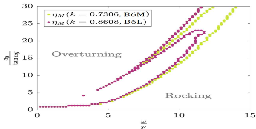
Figure 7. Stability graph for a single sine wave acceleration excitation for blocks with \frac{h}{b} = 4.5 : B6M and B6L.
