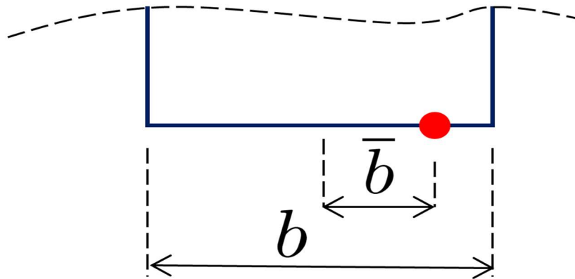
Figure 3. Impact position for calculating k needed in equation (10).
