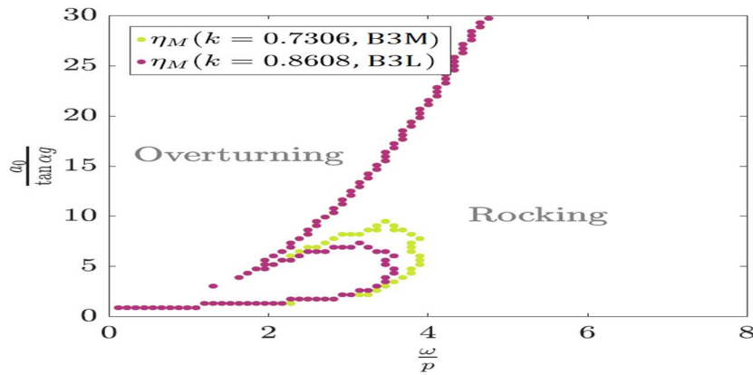
Figure 8. Stability graph for a single cosine wave acceleration excitation for blocks with \frac{h}{b} = 2.25 : B3M and B3L.
