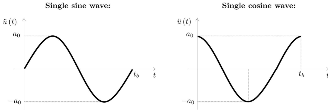
Figure 2. Ground acceleration functions examined.
