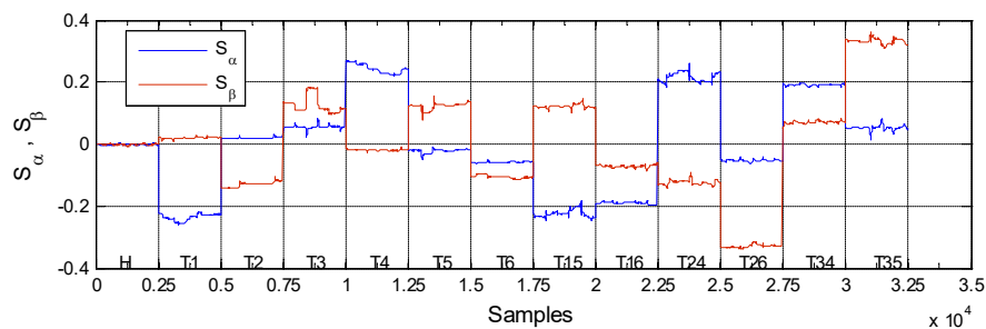
Figure 4. Feature extraction under open circuit switch fault occurrence.
