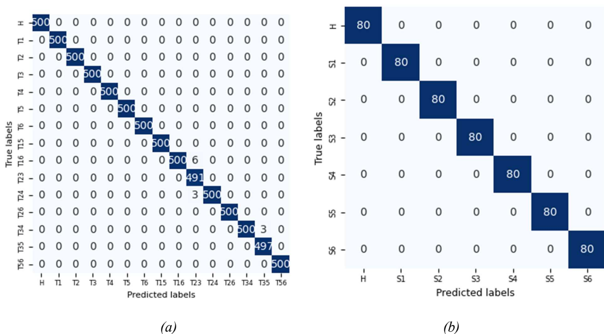
Figure 9. Confusion matrix for test data (a) open-switches and (b) short-circuit cases.
