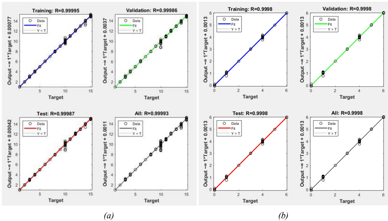
Figure 8. Behavior of the MLP during training, validation and testing process for (a) open-switches and (b) short-circuit cases.
