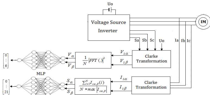
Figure 3. Proposed fault diagnosis system.
