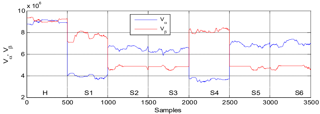
Figure 5. Feature extraction under short-circuit switch fault occurrence.
