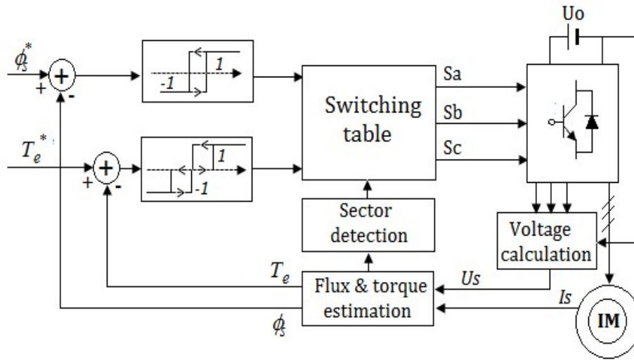
Figure 1. Basic DTC block diagram.
