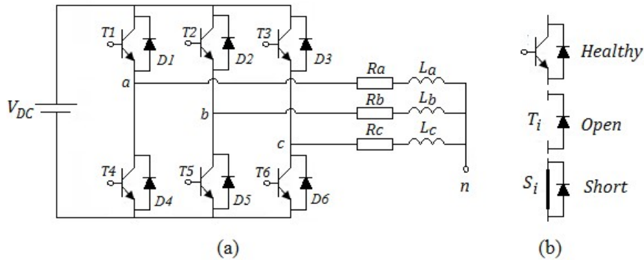
Figure 2. Diagram of a VSI feeding three-phase induction motor (a) and typical faults (b).
