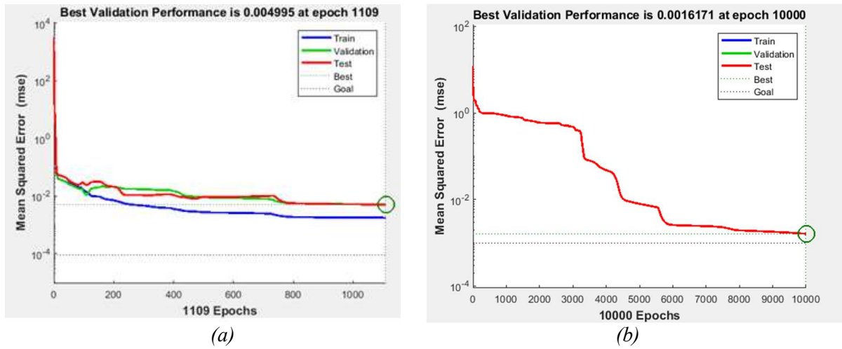
Figure 7. Training process for (a) open-switches and (b) short-circuit cases.
