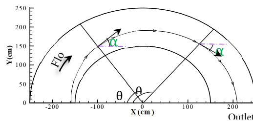
Fig. 20. Measurement of the streamlines' angle of deviation.
