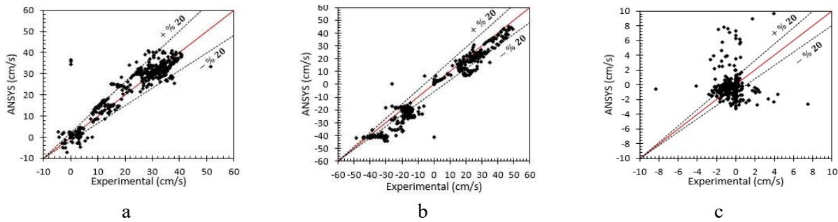
Fig. 6. A comparison between a) tangential, b) radial, and c) vertical velocity data in both numerical and experimental models
