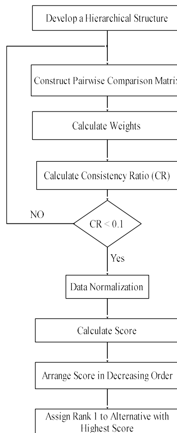
Figure 2. Flow Chart of AHP.
