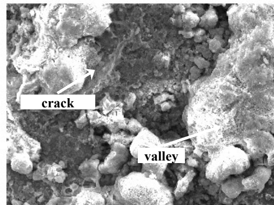
(b) Corroded specimen, magnified 500×
