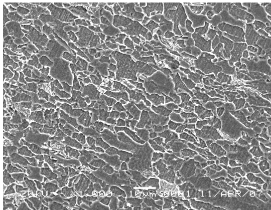
(a) Without corrosion, magnified 1000×
