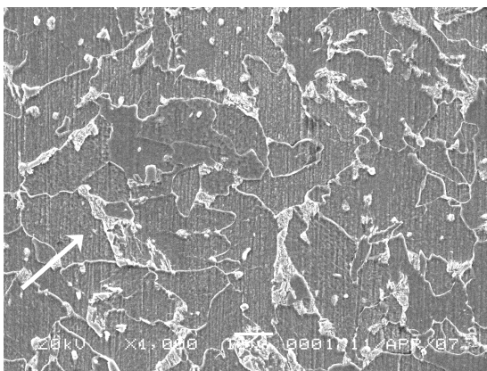
(a) Normal specimen, magnified 1000 ×
