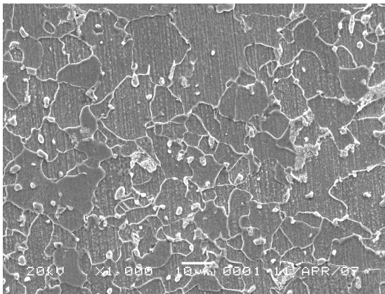
(a) Normal l specimen, magnified 1000 ×
