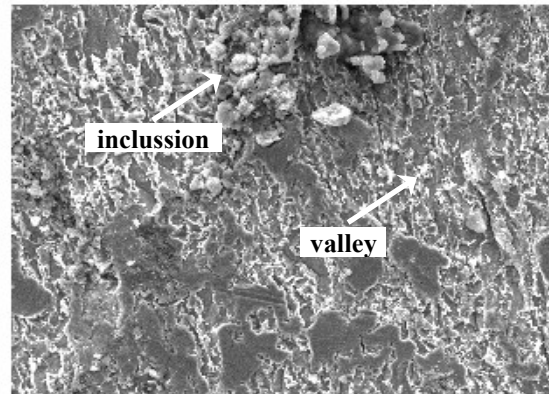
(b) Corroded specimen, magnified 500×
