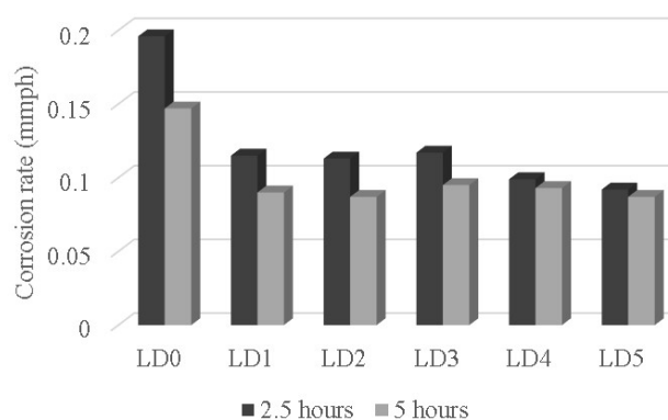
Figure 6. Corrosion rate vs duration of corrosion testing.
