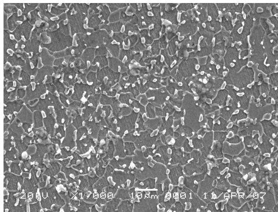
(a) Without corrosion, magnified 1000 ×
