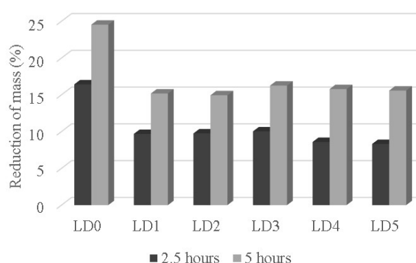
Figure 3. Mass reduction VS duration of corrosion testing.
