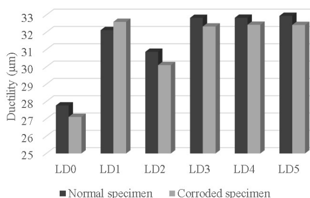
Figure 4. The ductility of normal and corroded specimens.
