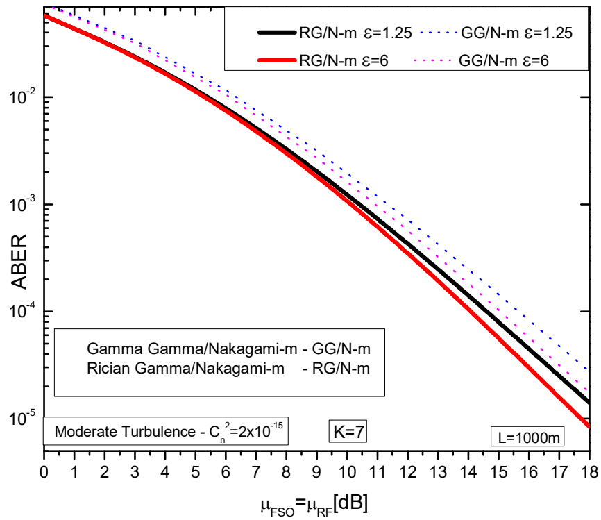
Figure 3. ABER relationship when using hybrid RF/FSO systems with Rician-Gamma distribution and Nakagami- m fading, and Gamma-Gamma distribution and Nakagami- m fading, depending on pointing error.
