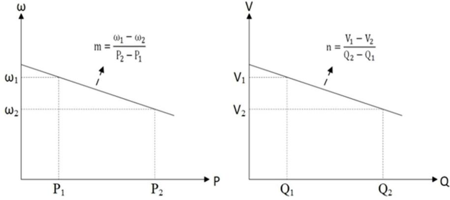
Figure 3. Droop characteristic.
